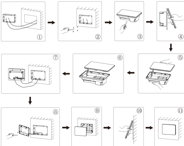
Fig.1.7 Installation Diagram
